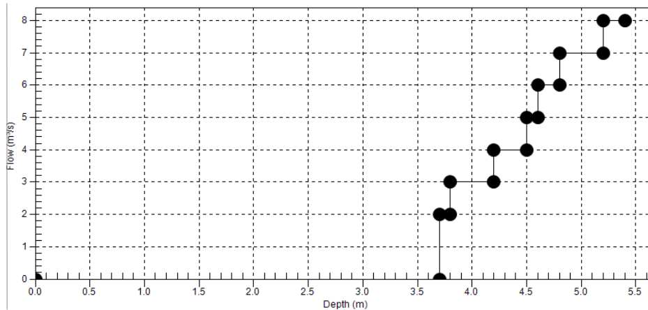
Fig. 2. Pump curve of Trabek station programmed in PCSWMM, showing forebay depth at which individual pumps are turned on
