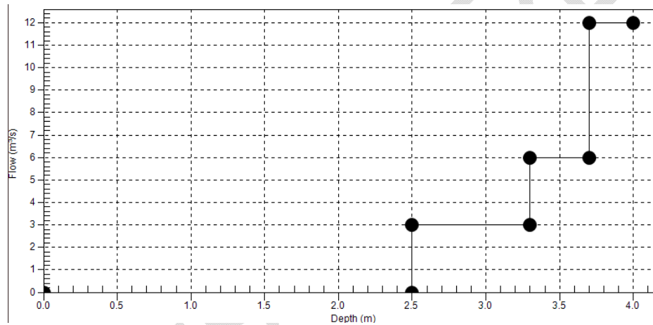
Fig. 3. Pump curve of Tumpun station programmed in PCSWMM, showing forebay depth at which individual pumps are turned on
